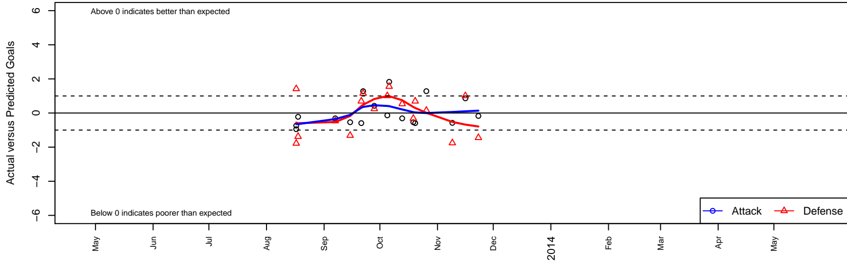
Eagles SC White G01 Dots are actual minus expected GF (blue circles) and GA (red triangles). Blue line is smoothed change in attack strength. Red is smoothed change in defense strength.
